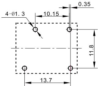
Mounting Dimensions安装尺寸
