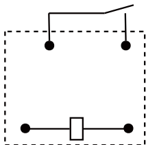
Internal Connections接线图
